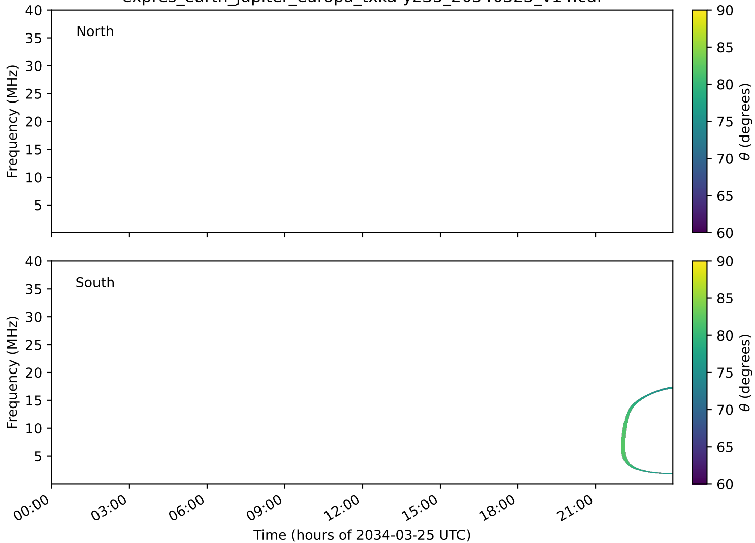
expres_earth_jupiter_europa_txka-y235_20340325_v14.cdf
