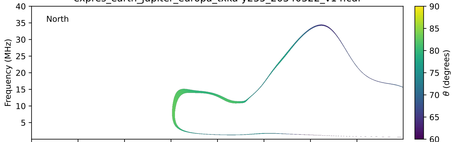
expres_earth_jupiter_europa_txka-y235_20340322_v14.cdf
