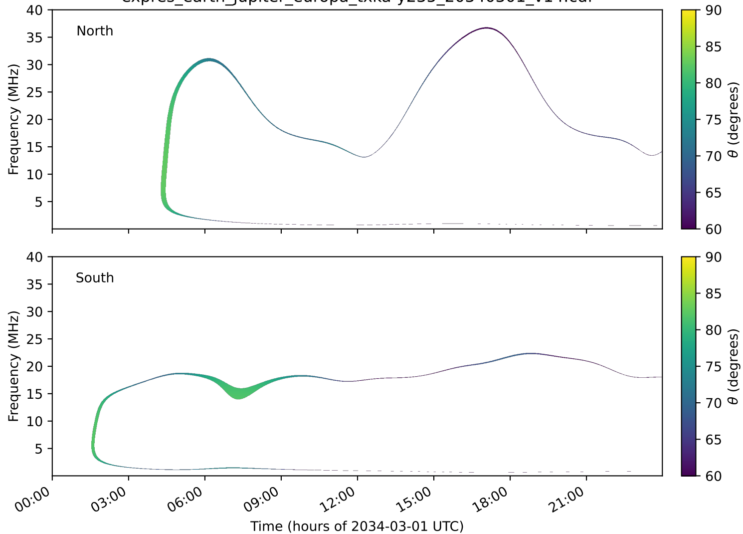
expres_earth_jupiter_europa_txka-y235_20340301_v14.cdf
