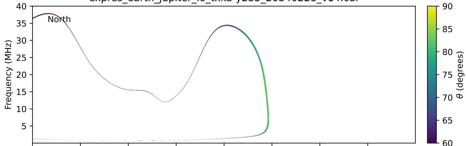
expres_earth_jupiter_io_txka-y235_20340228_v14.cdf
