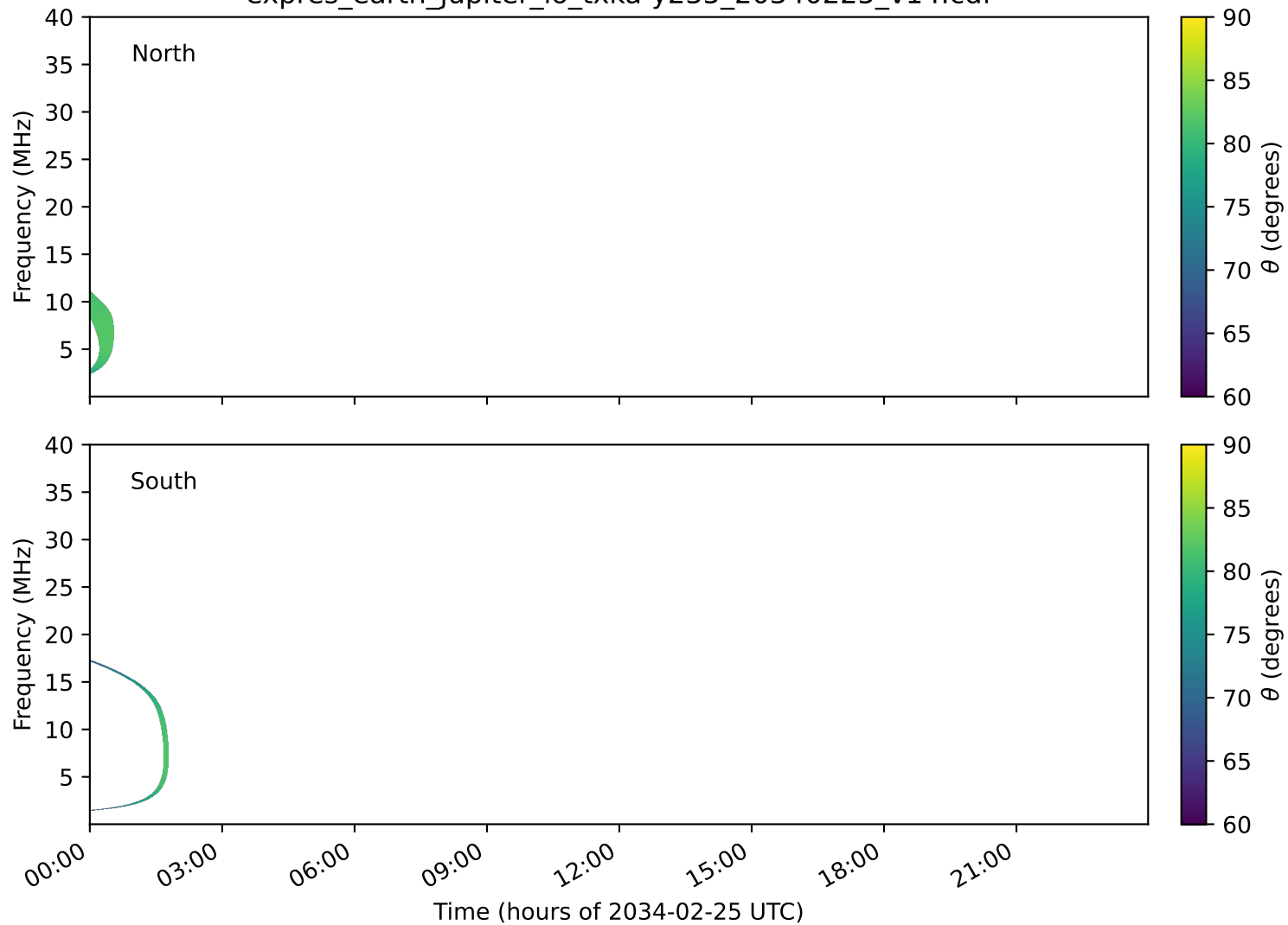
expres_earth_jupiter_io_txka-y235_20340225_v14.cdf
