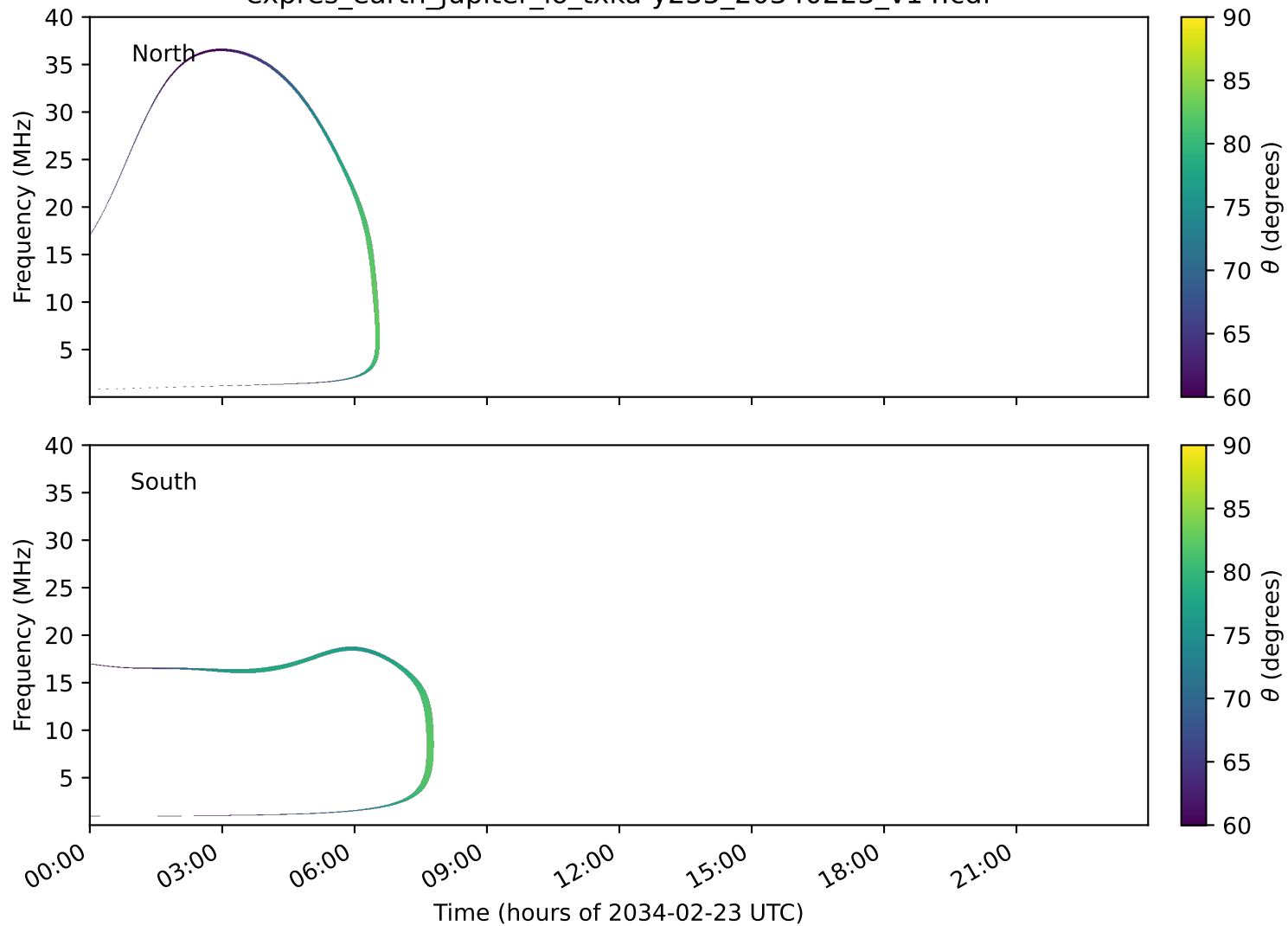
expres_earth_jupiter_io_txka-y235_20340223_v14.cdf
