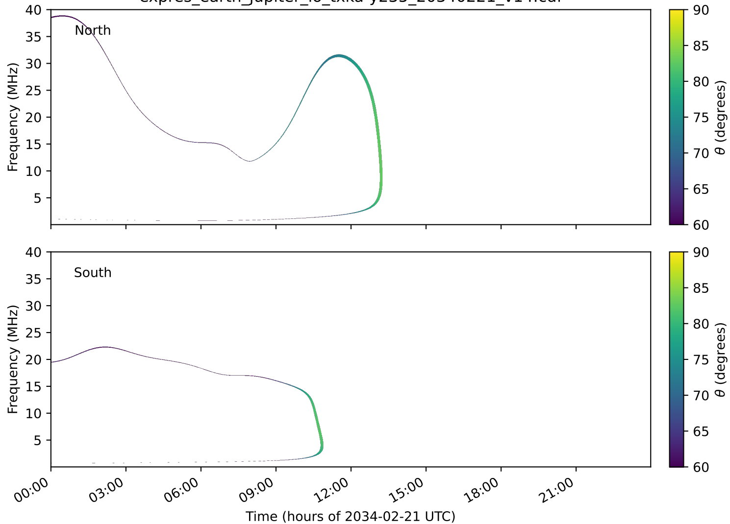
expres_earth_jupiter_io_txka-y235_20340221_v14.cdf
