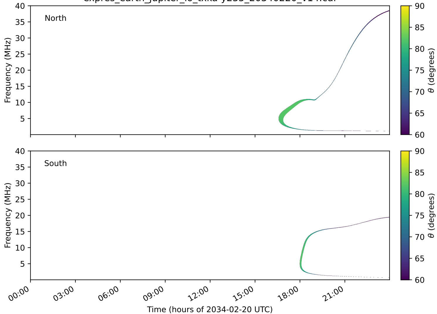
expres_earth_jupiter_io_txka-y235_20340220_v14.cdf
