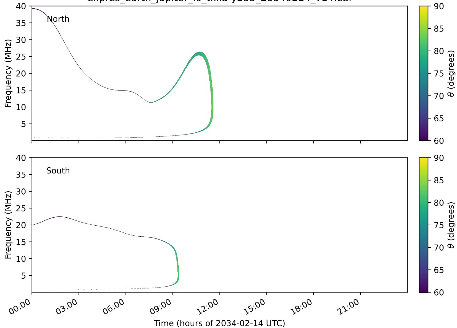
expres_earth_jupiter_io_txka-y235_20340214_v14.cdf
