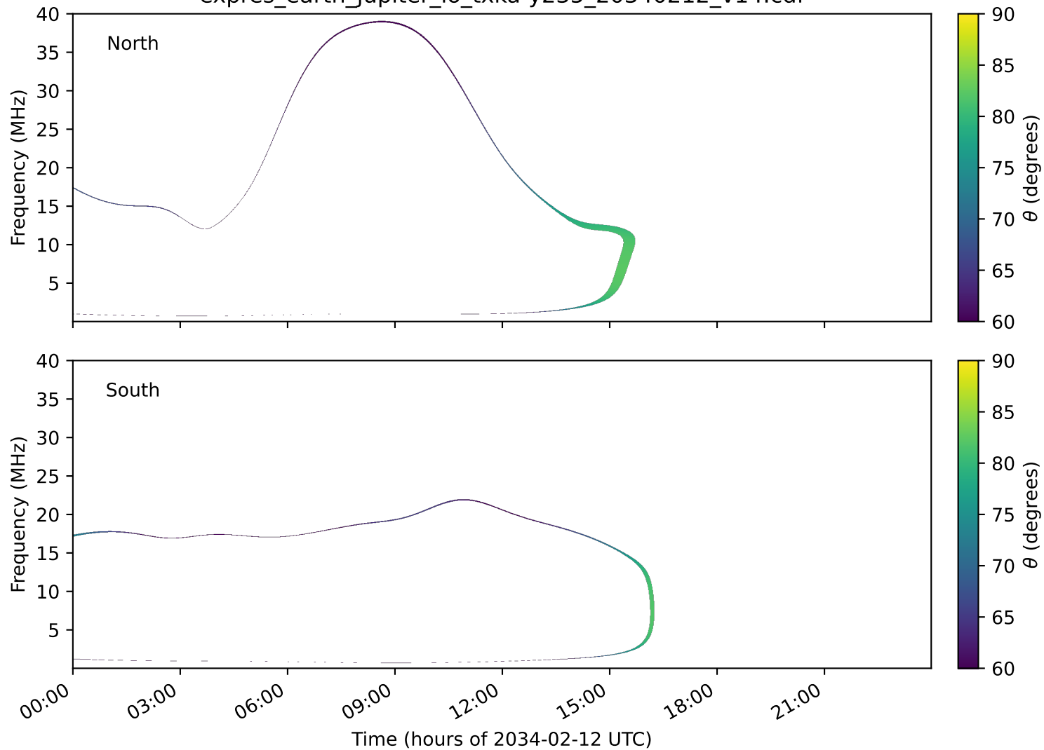
expres_earth_jupiter_io_txka-y235_20340212_v14.cdf
