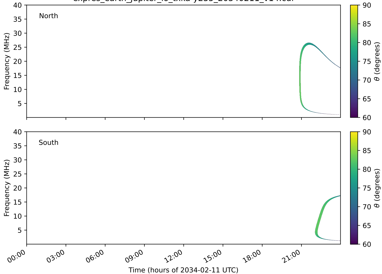
expres_earth_jupiter_io_txka-y235_20340211_v14.cdf
