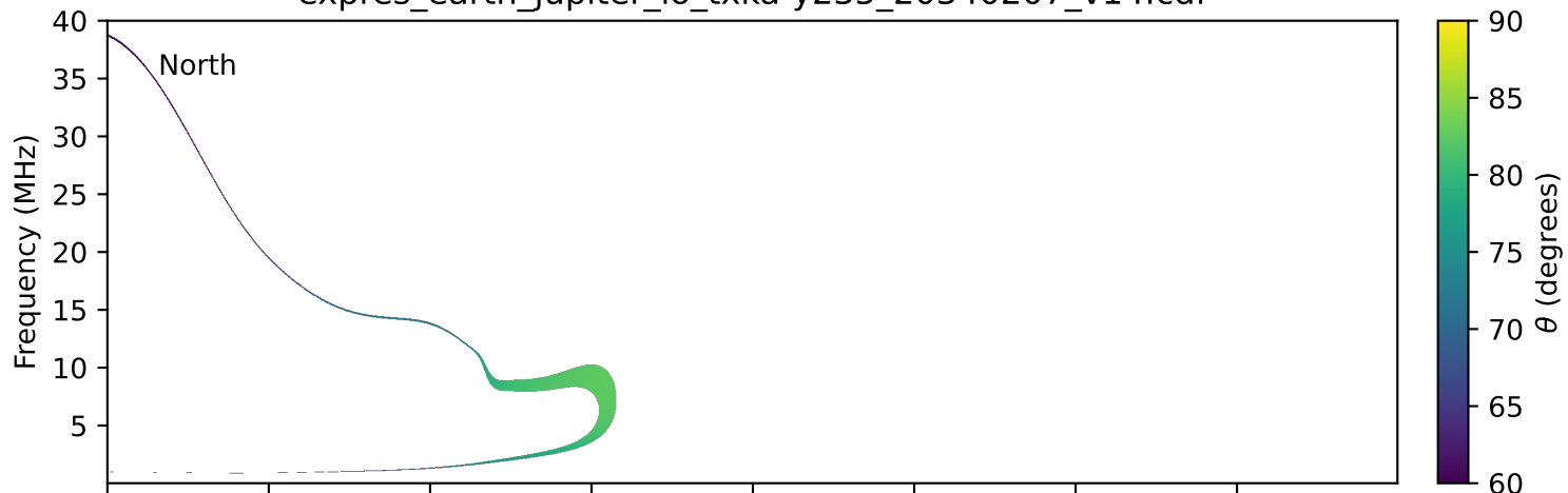
expres_earth_jupiter_io_txka-y235_20340207_v14.cdf
