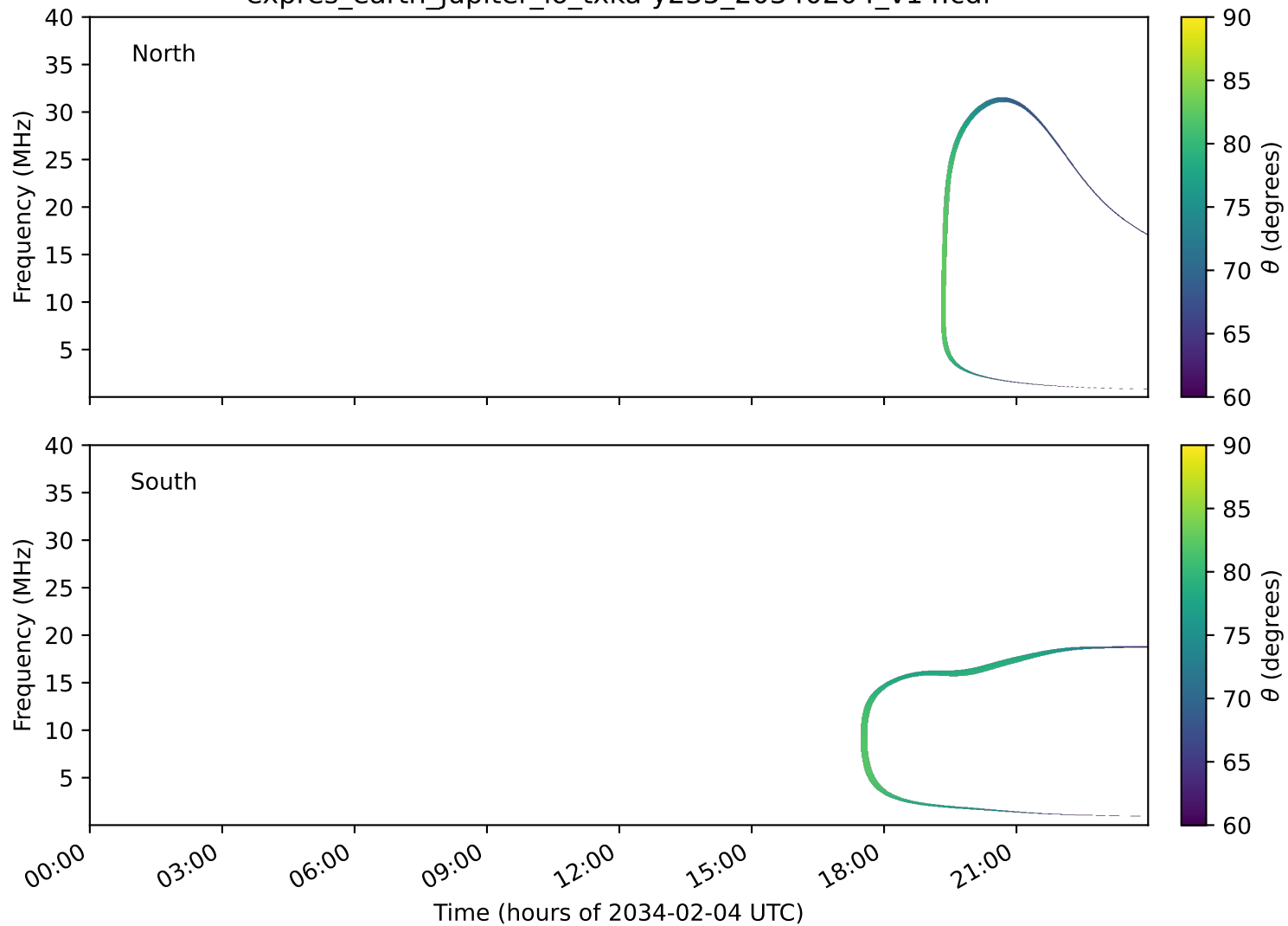
expres_earth_jupiter_io_txka-y235_20340204_v14.cdf
