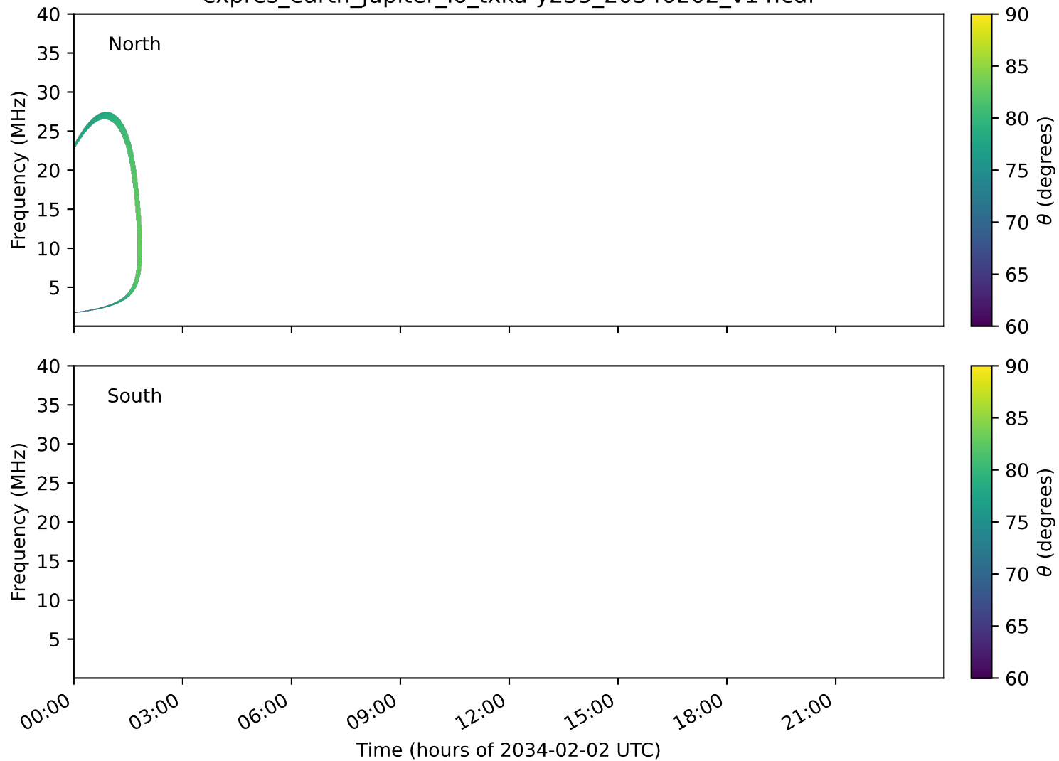
expres_earth_jupiter_io_txka-y235_20340202_v14.cdf
