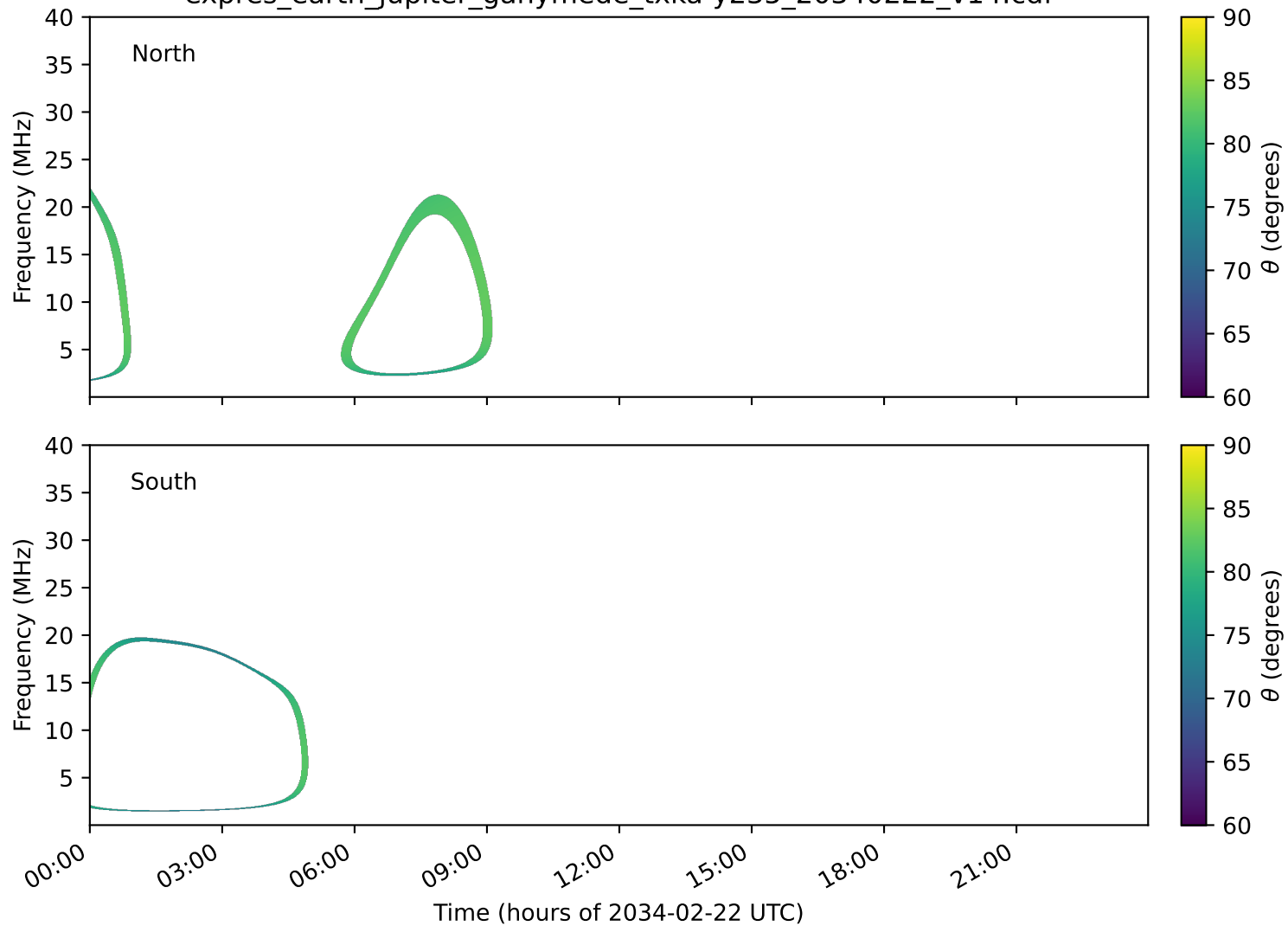
expres_earth_jupiter_ganymede_txka-y235_20340222_v14.cdf
