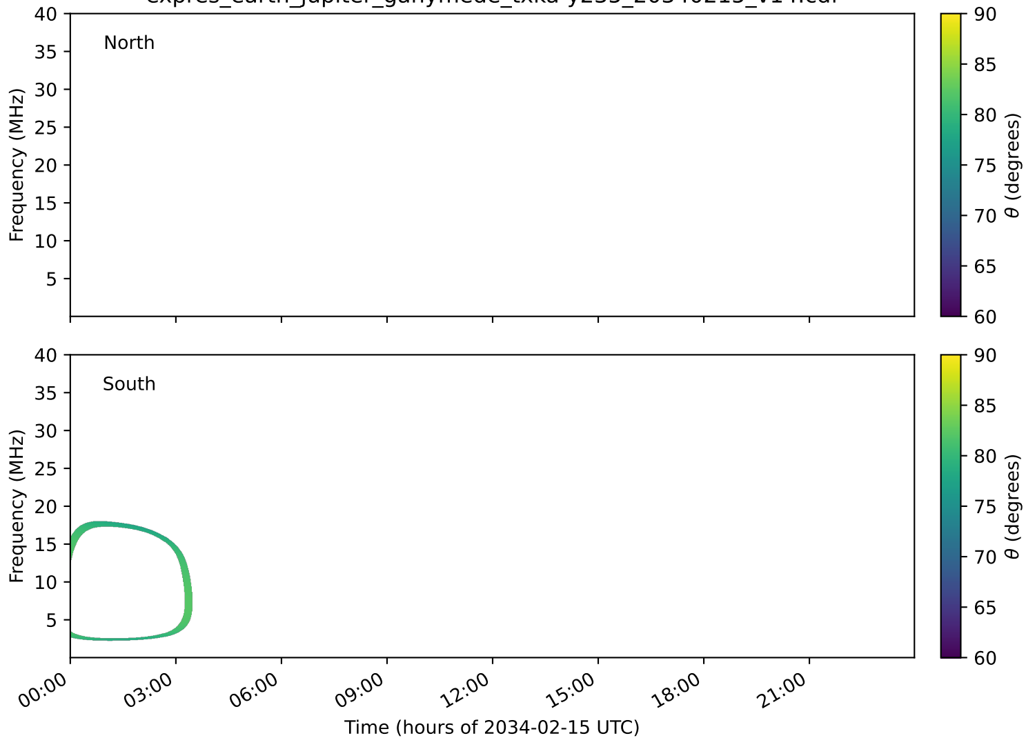
expres_earth_jupiter_ganymede_txka-y235_20340215_v14.cdf
