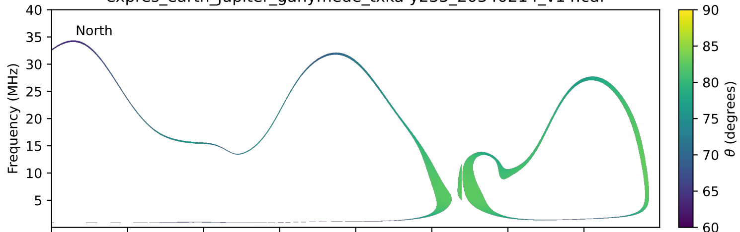
expres_earth_jupiter_ganymede_txka-y235_20340214_v14.cdf
