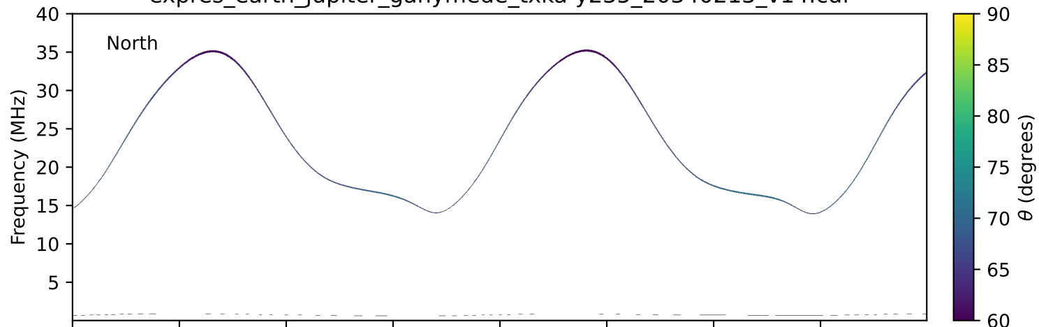
expres_earth_jupiter_ganymede_txka-y235_20340213_v14.cdf
