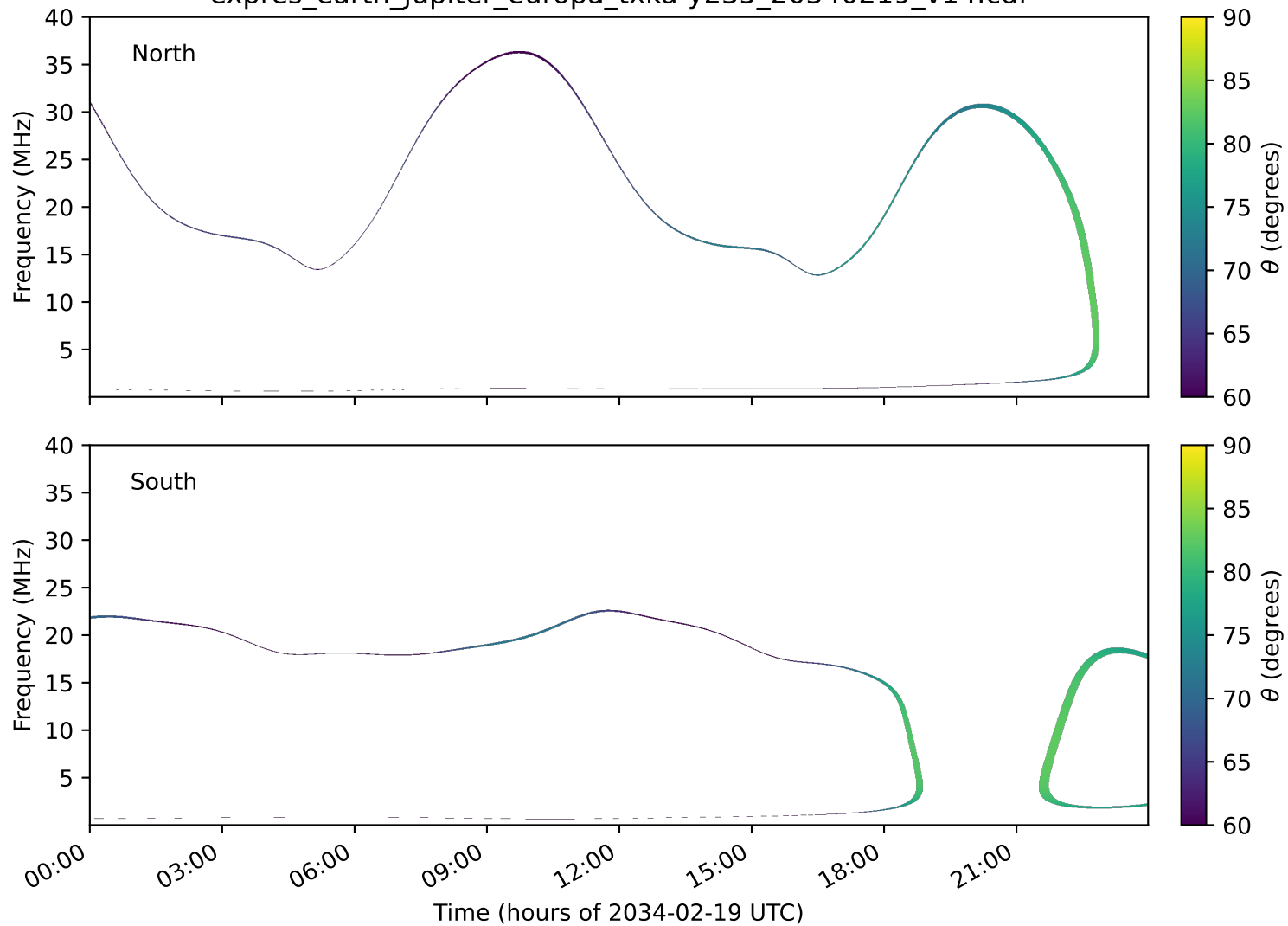
expres_earth_jupiter_europa_txka-y235_20340219_v14.cdf
