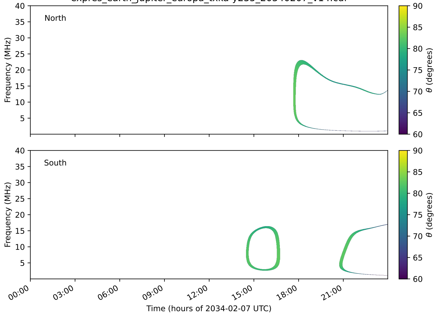
expres_earth_jupiter_europa_txka-y235_20340207_v14.cdf
