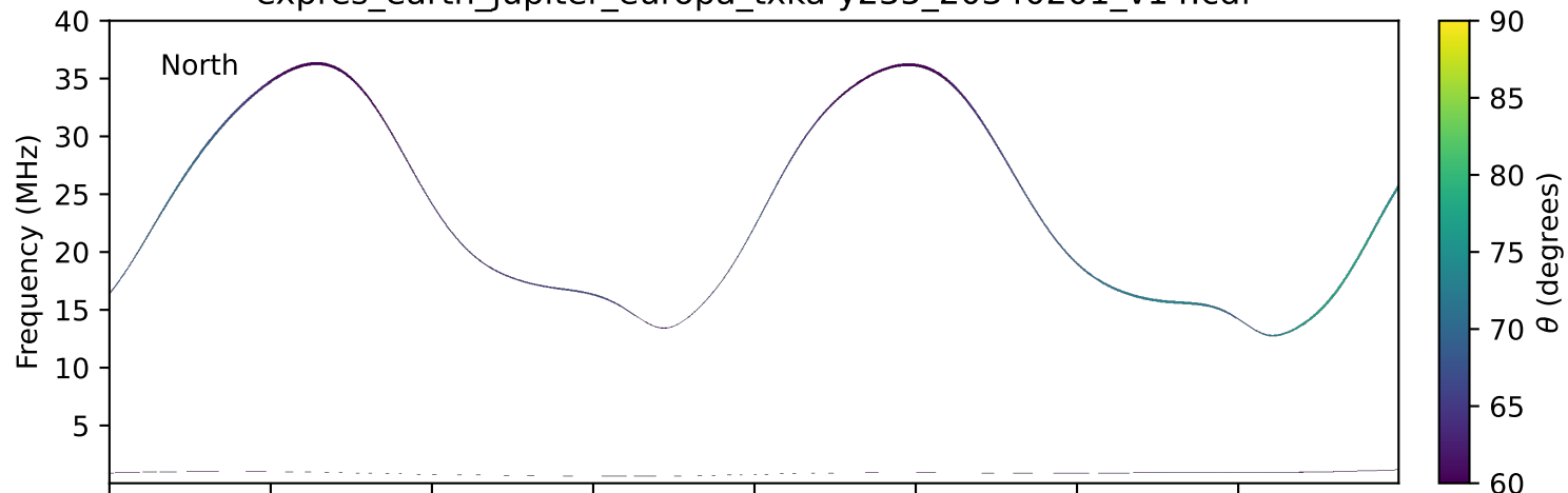
expres_earth_jupiter_europa_txka-y235_20340201_v14.cdf
