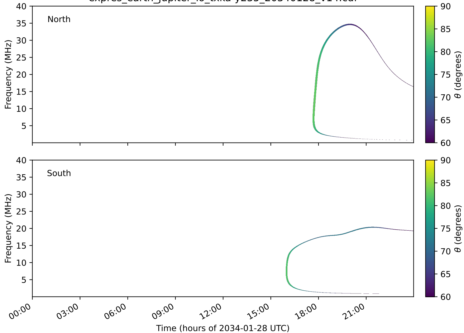
expres_earth_jupiter_io_txka-y235_20340128_v14.cdf
