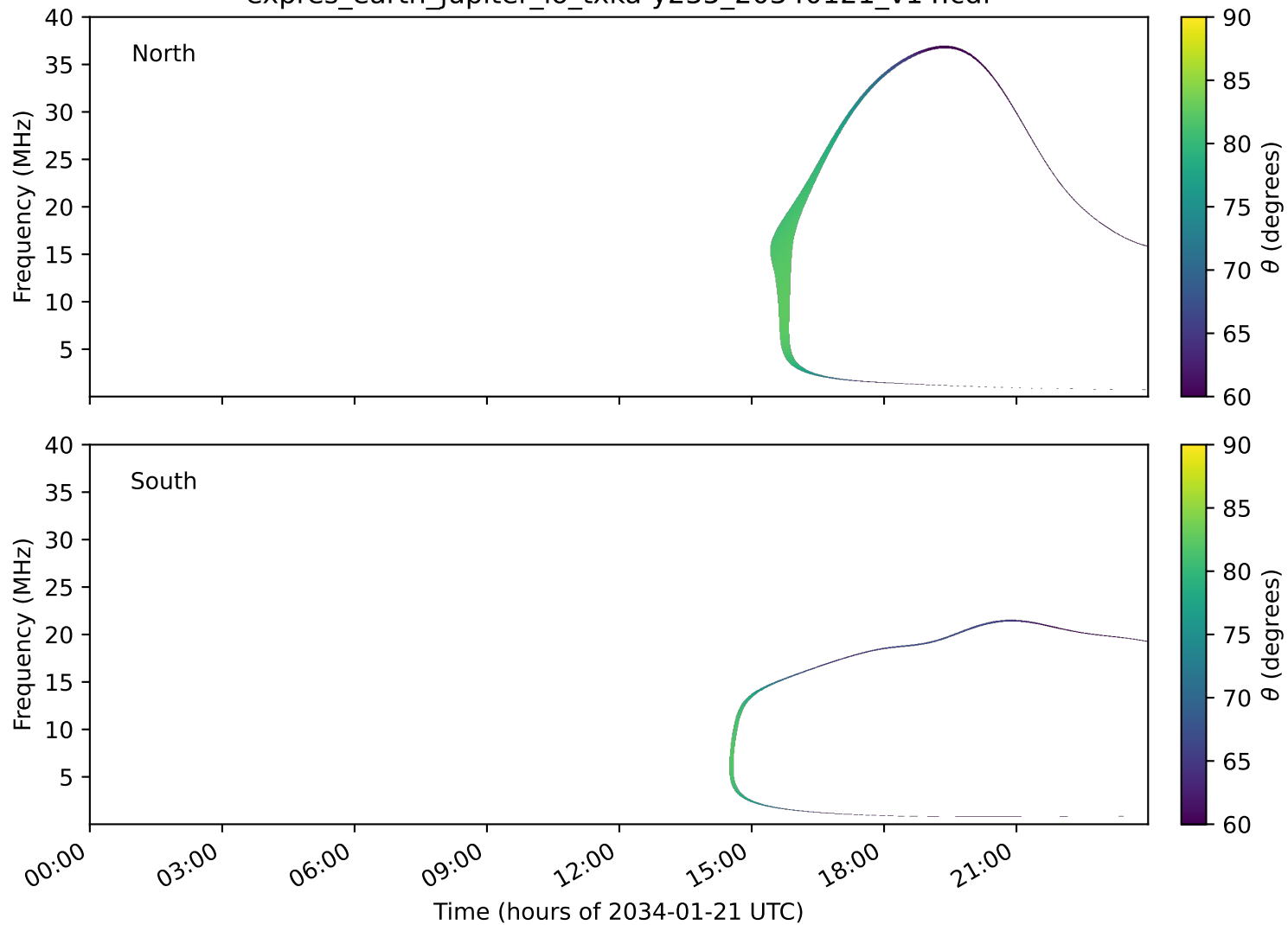
expres_earth_jupiter_io_txka-y235_20340121_v14.cdf
