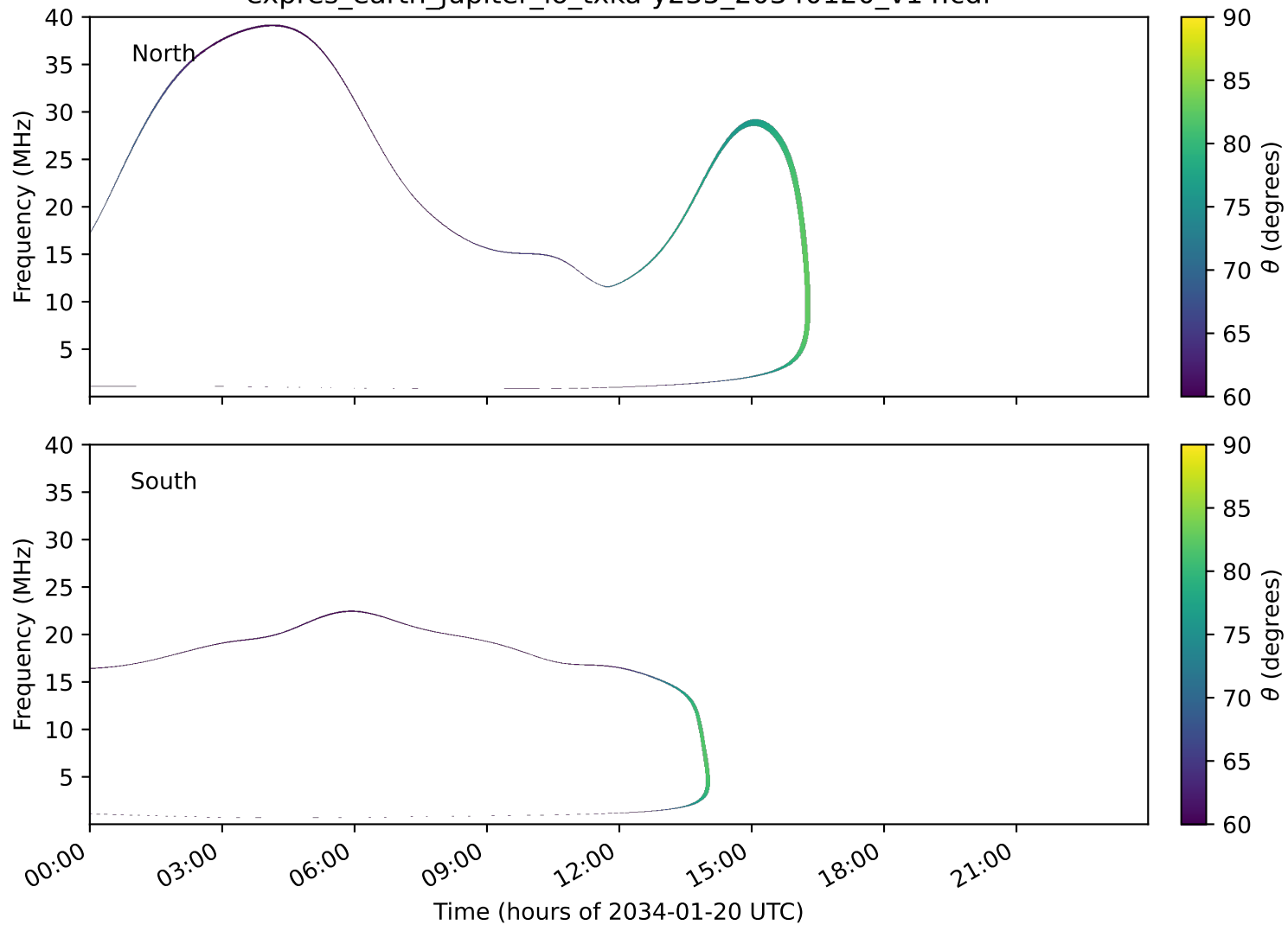
expres_earth_jupiter_io_txka-y235_20340120_v14.cdf
