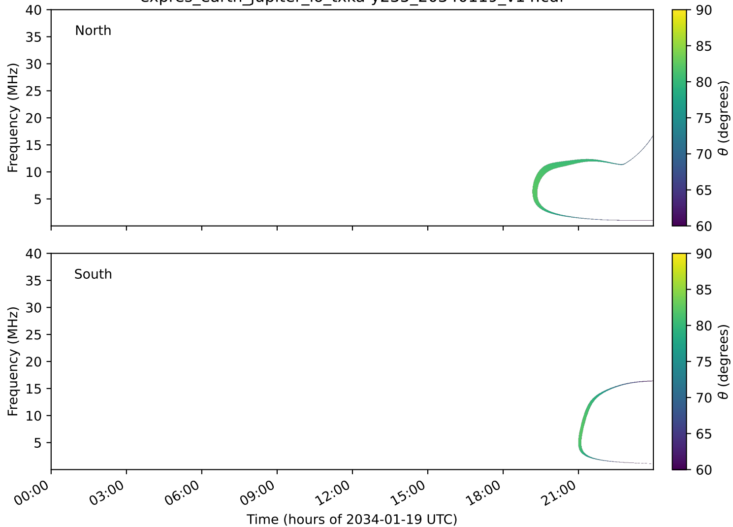
expres_earth_jupiter_io_txka-y235_20340119_v14.cdf
