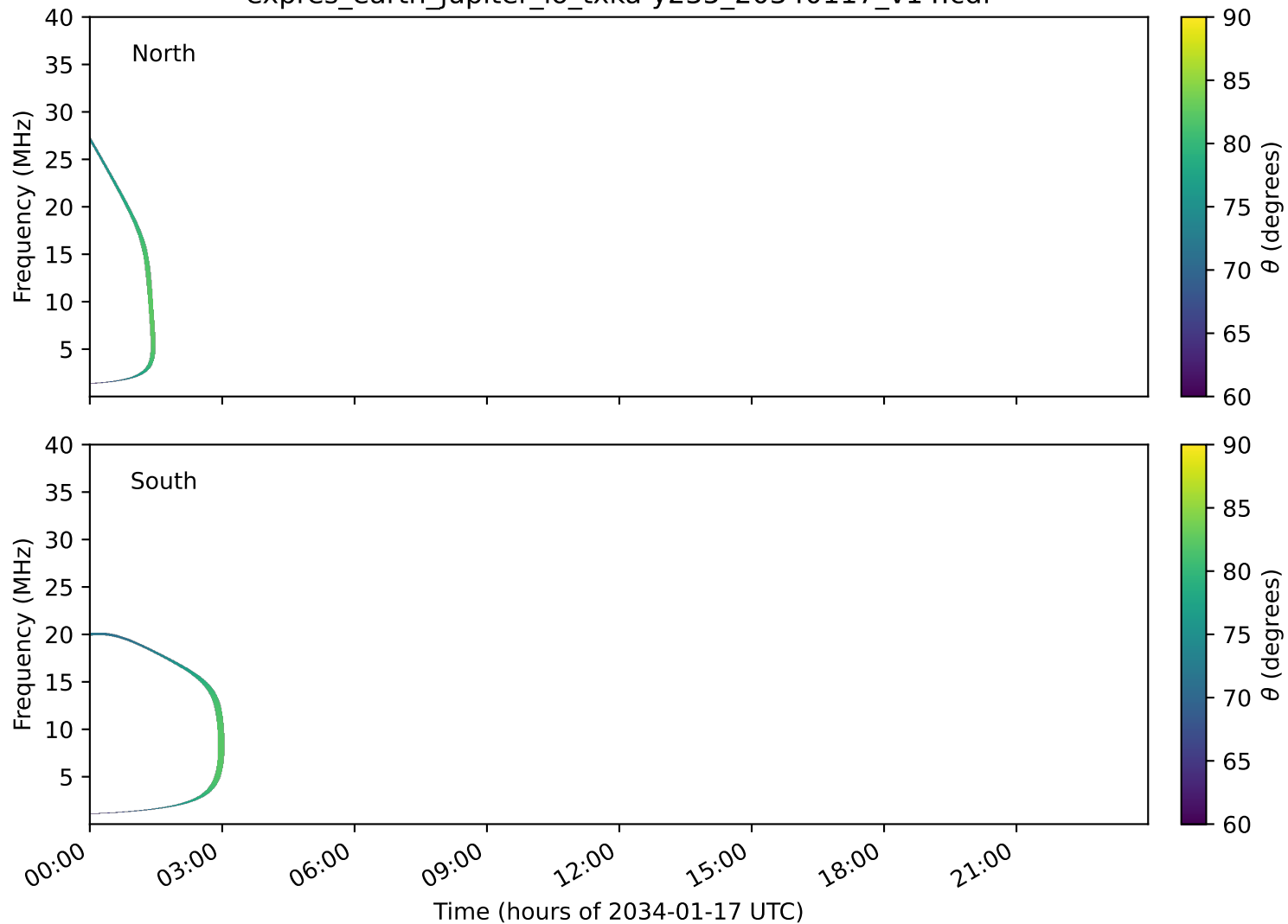
expres_earth_jupiter_io_txka-y235_20340117_v14.cdf
