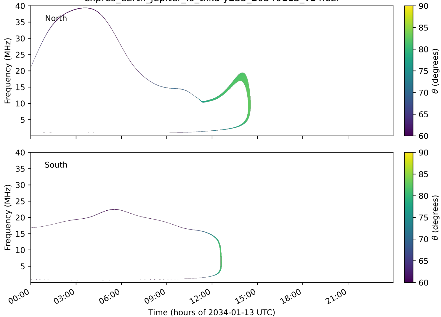
expres_earth_jupiter_io_txka-y235_20340113_v14.cdf
