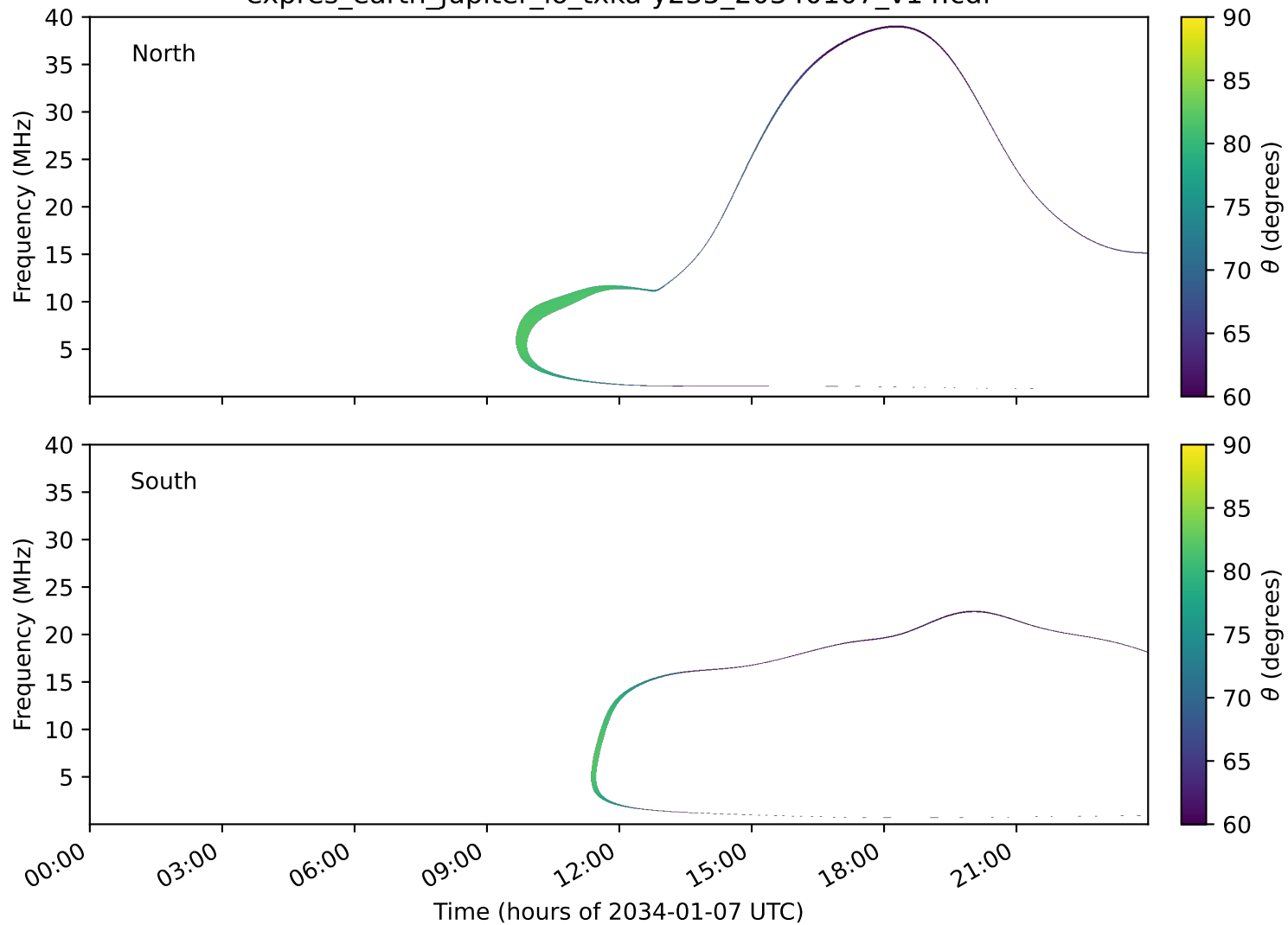
expres_earth_jupiter_io_txka-y235_20340107_v14.cdf
