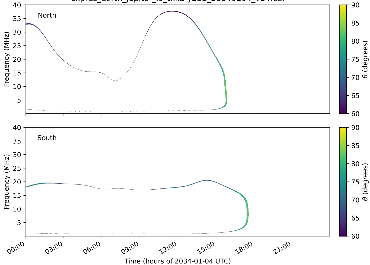
expres_earth_jupiter_io_txka-y235_20340104_v14.cdf
