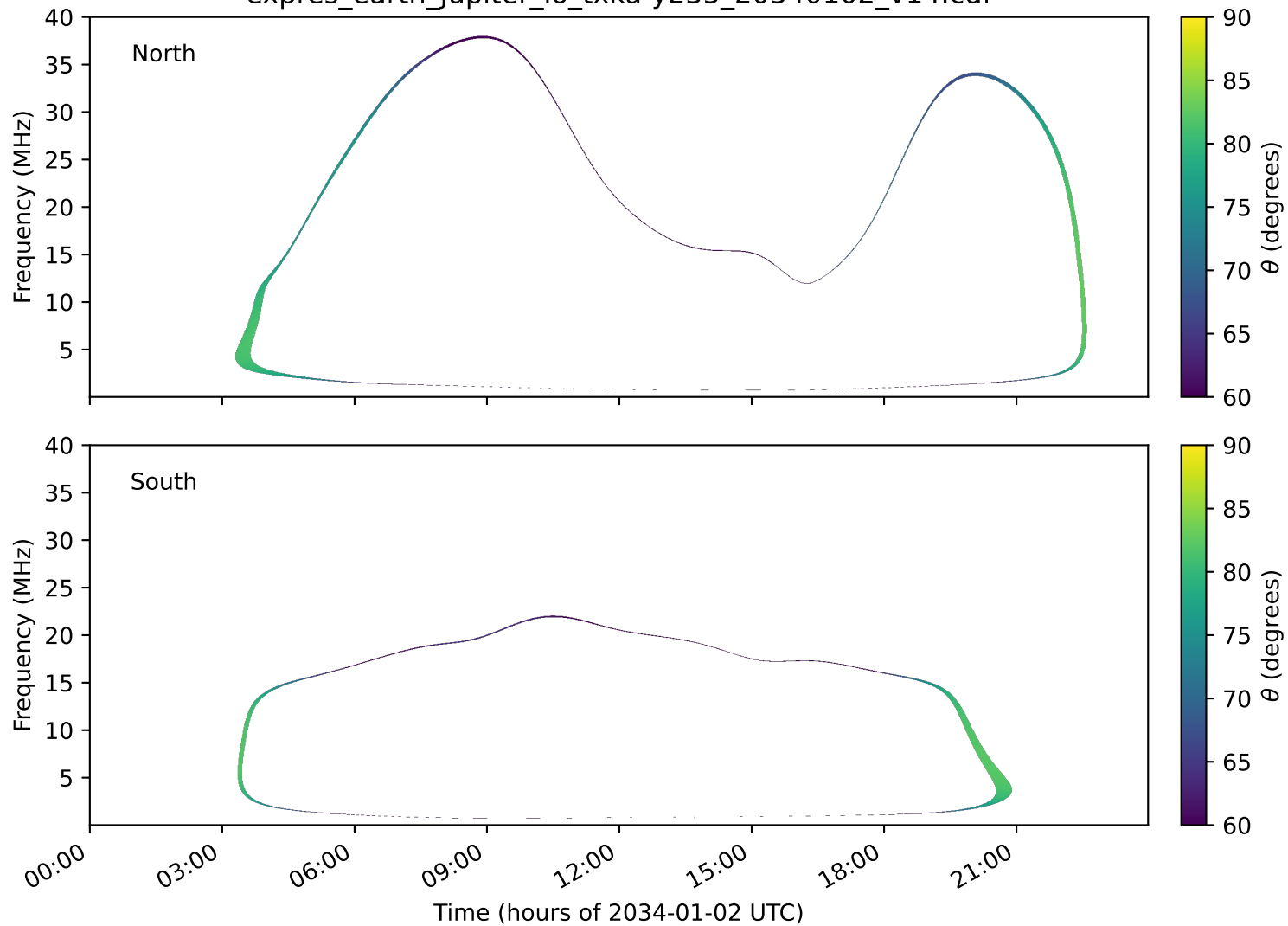
expres_earth_jupiter_io_txka-y235_20340102_v14.cdf
