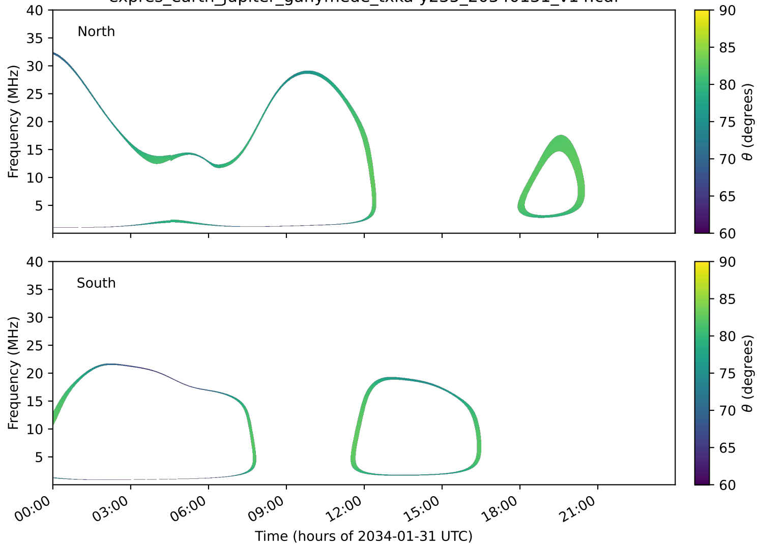
expres_earth_jupiter_ganymede_txka-y235_20340131_v14.cdf
