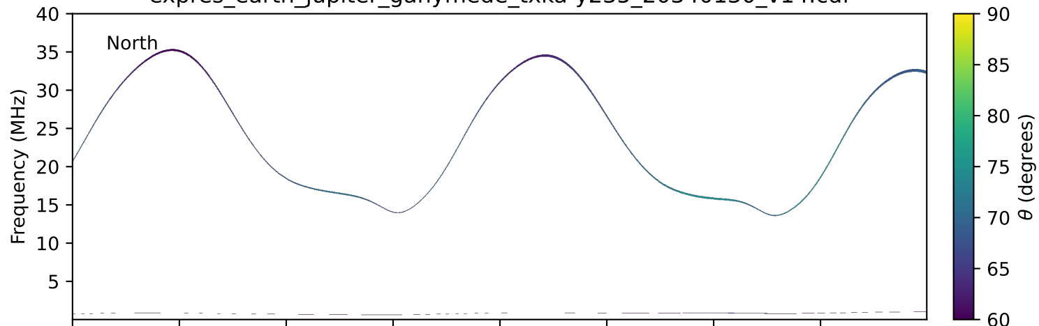
expres_earth_jupiter_ganymede_txka-y235_20340130_v14.cdf
