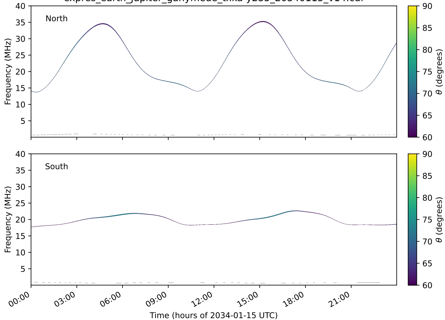
expres_earth_jupiter_ganymede_txka-y235_20340115_v14.cdf
