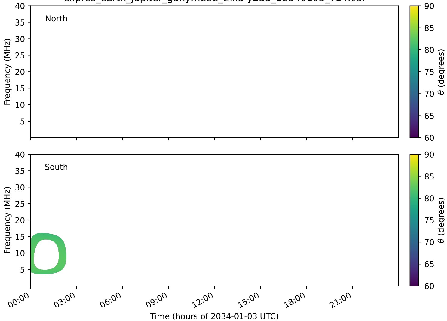
expres_earth_jupiter_ganymede_txka-y235_20340103_v14.cdf
