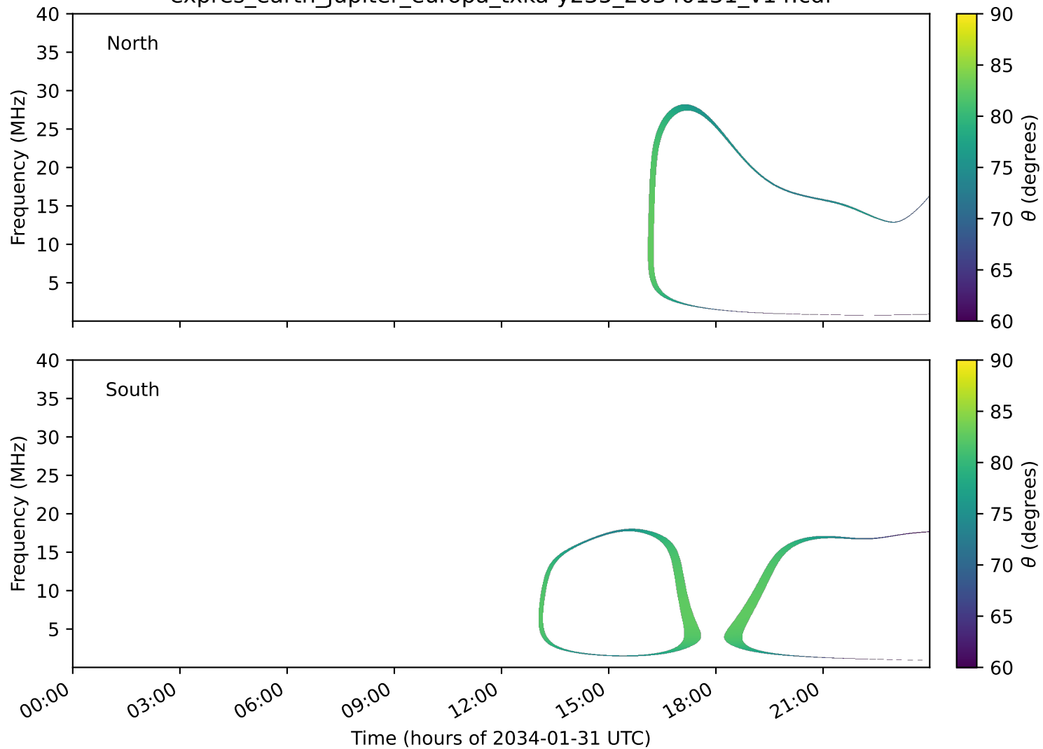
expres_earth_jupiter_europa_txka-y235_20340131_v14.cdf
