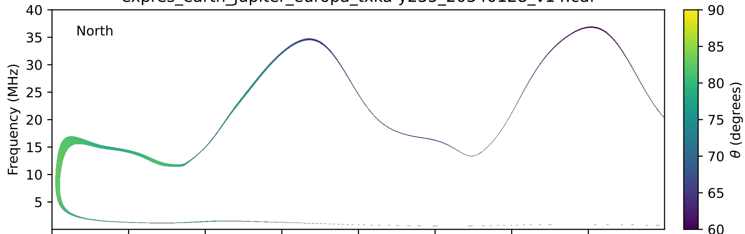
expres_earth_jupiter_europa_txka-y235_20340128_v14.cdf
