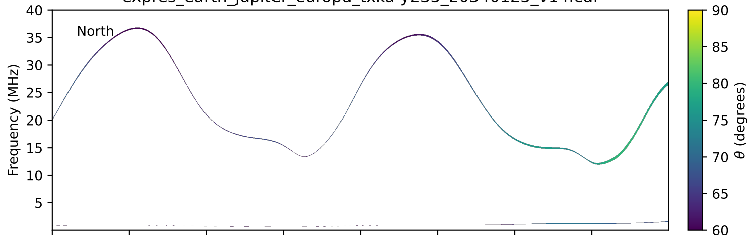
expres_earth_jupiter_europa_txka-y235_20340125_v14.cdf
