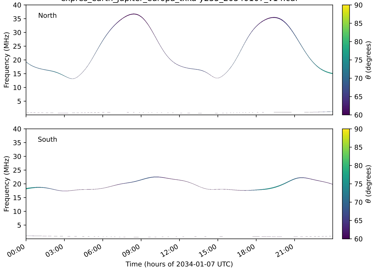
expres_earth_jupiter_europa_txka-y235_20340107_v14.cdf
