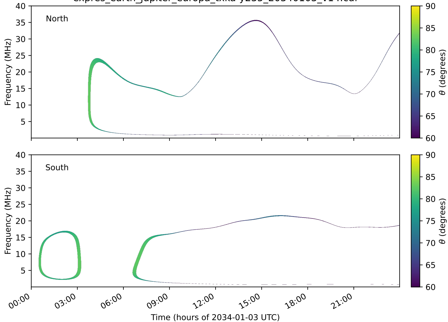
expres_earth_jupiter_europa_txka-y235_20340103_v14.cdf
