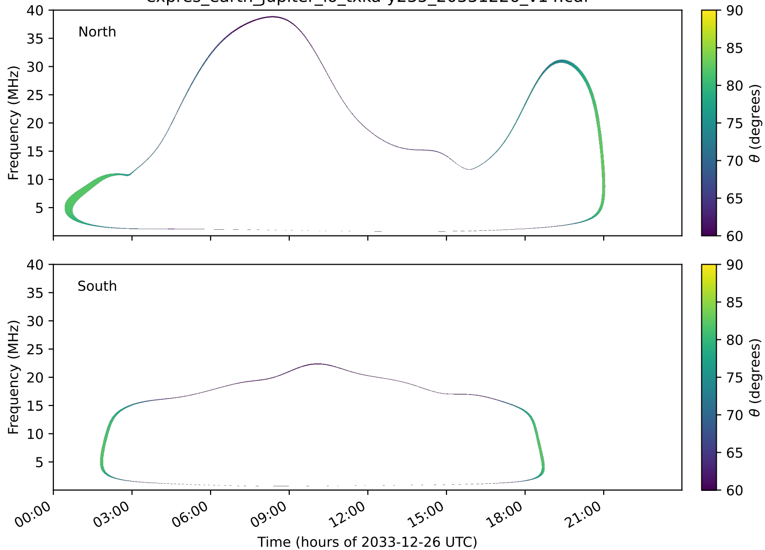
expres_earth_jupiter_io_txka-y235_20331226_v14.cdf
