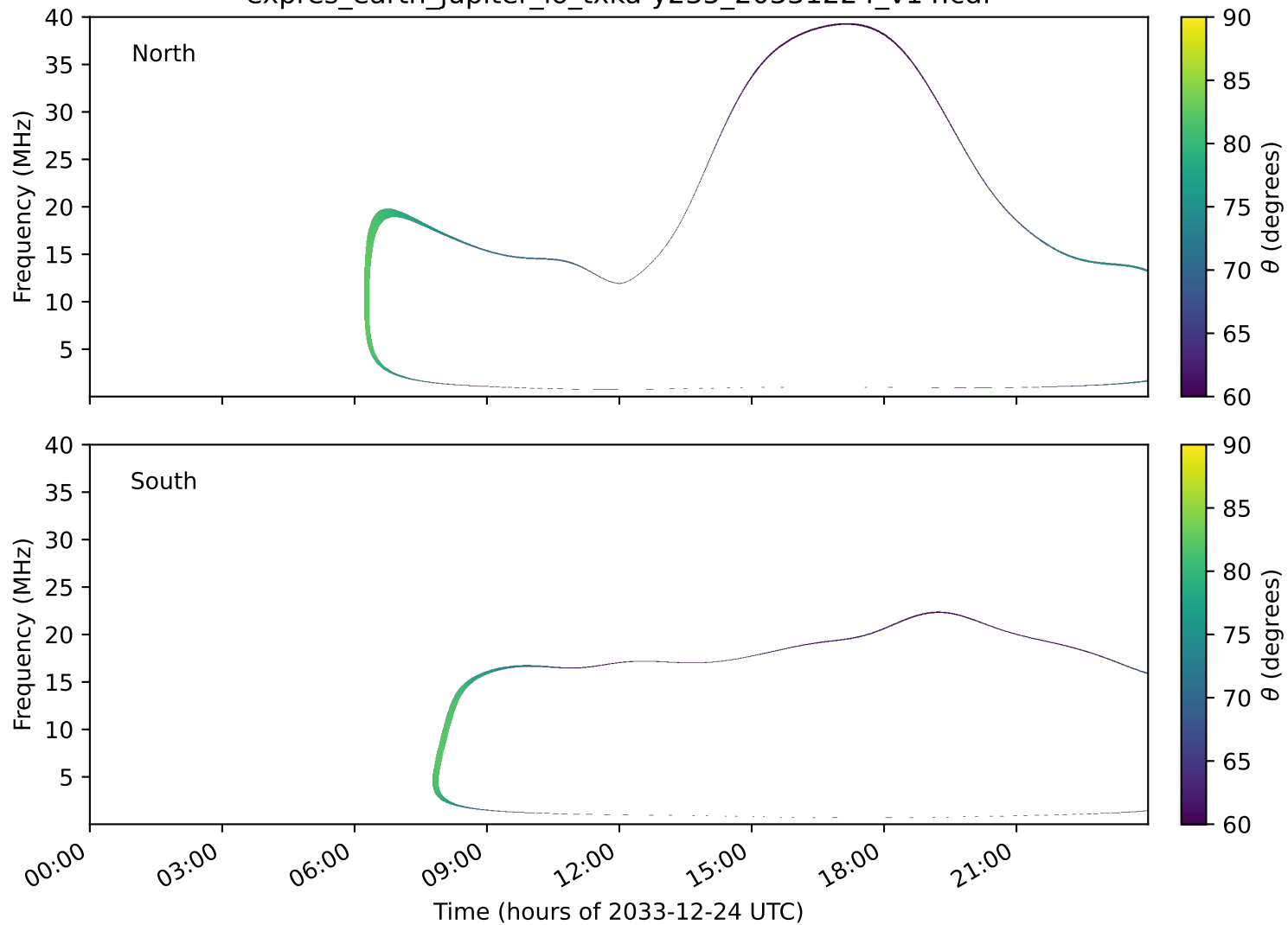
expres_earth_jupiter_io_txka-y235_20331224_v14.cdf
