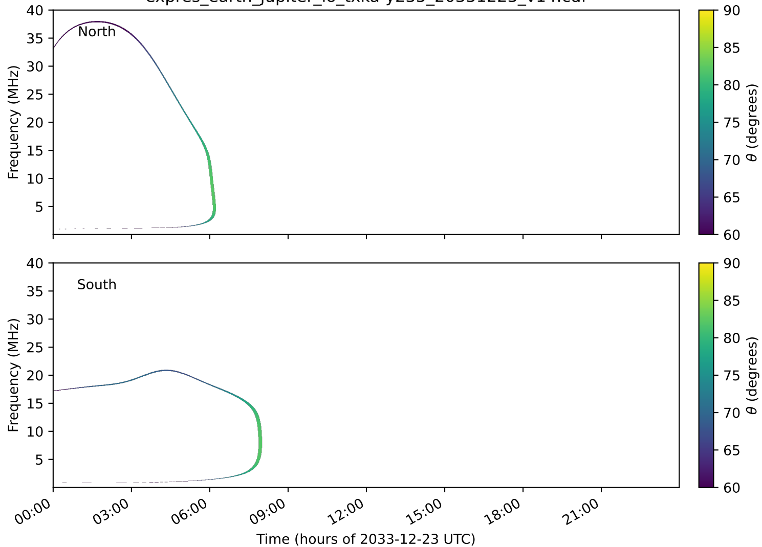
expres_earth_jupiter_io_txka-y235_20331223_v14.cdf
