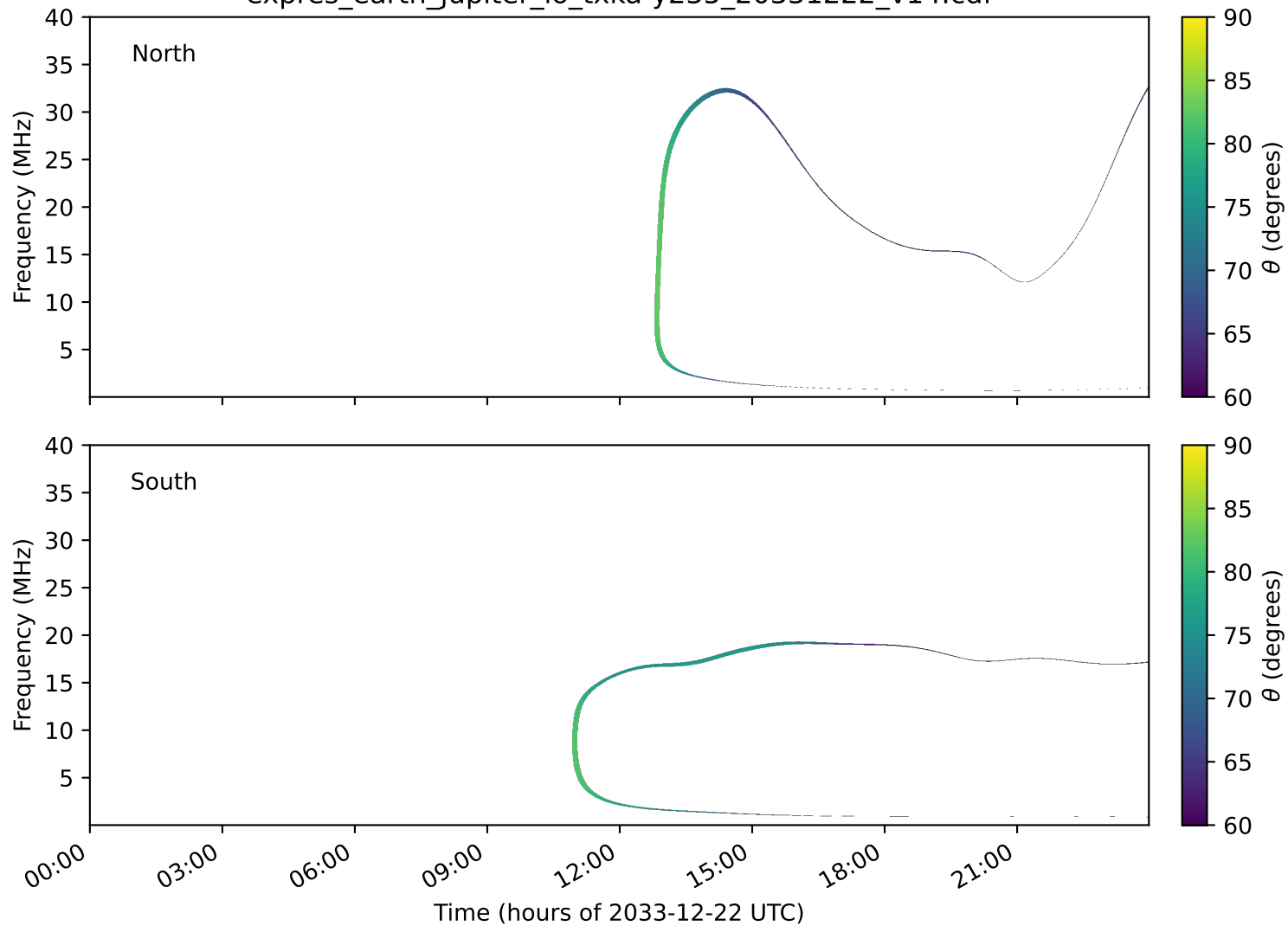
expres_earth_jupiter_io_txka-y235_20331222_v14.cdf
