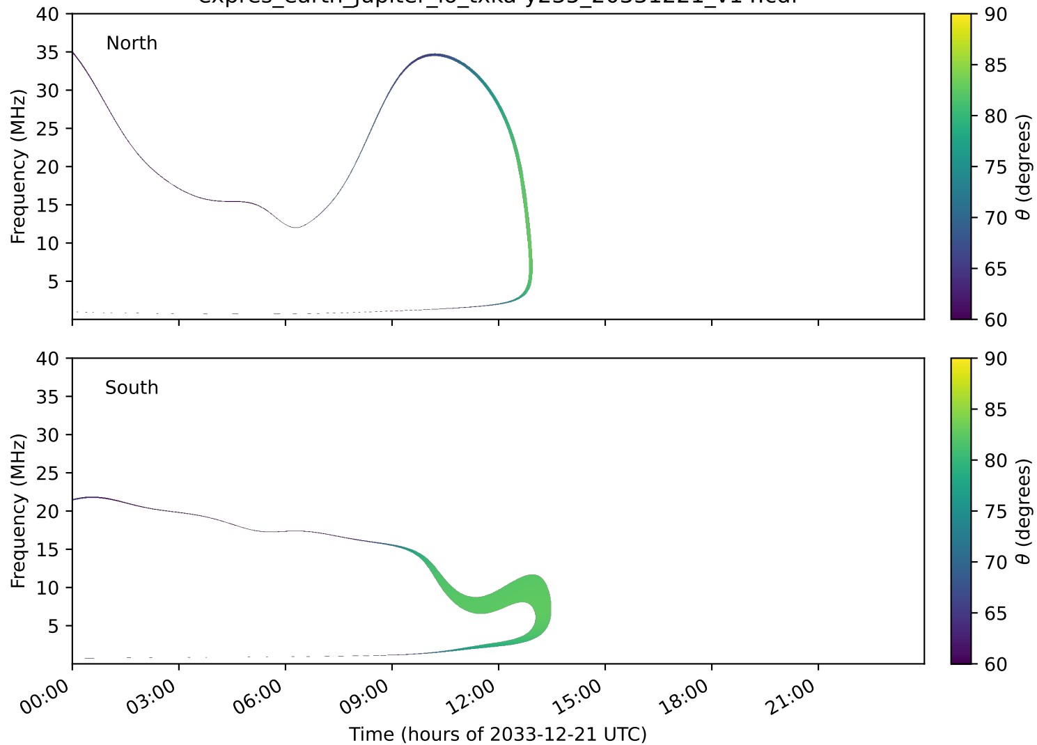
expres_earth_jupiter_io_txka-y235_20331221_v14.cdf
