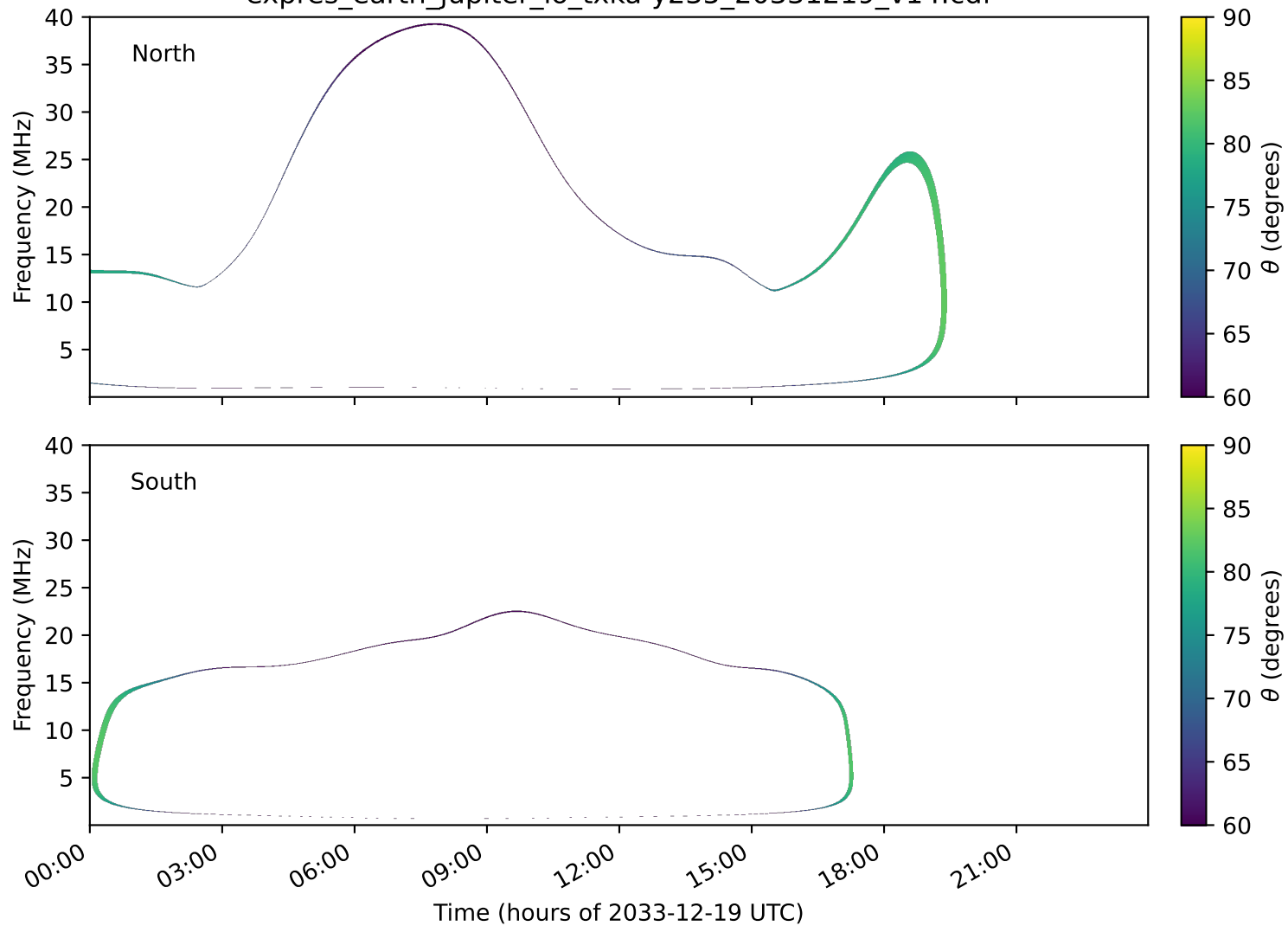
expres_earth_jupiter_io_txka-y235_20331219_v14.cdf
