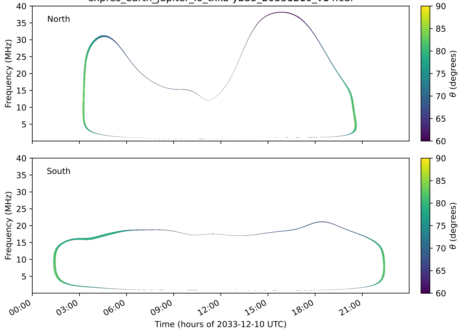
expres_earth_jupiter_io_txka-y235_20331210_v14.cdf
