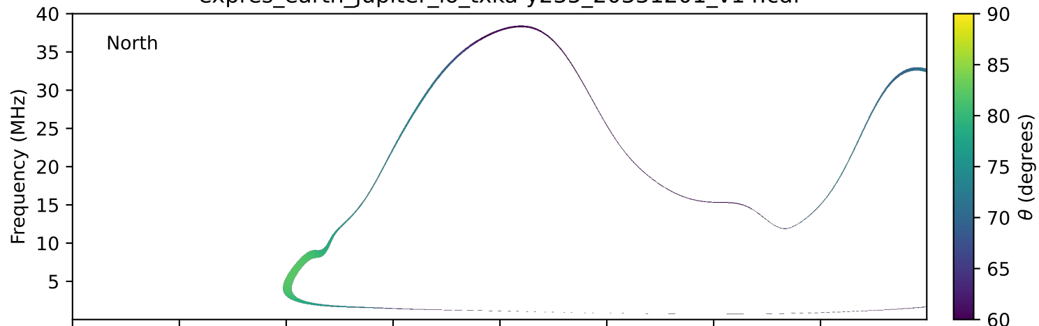
expres_earth_jupiter_io_txka-y235_20331201_v14.cdf
