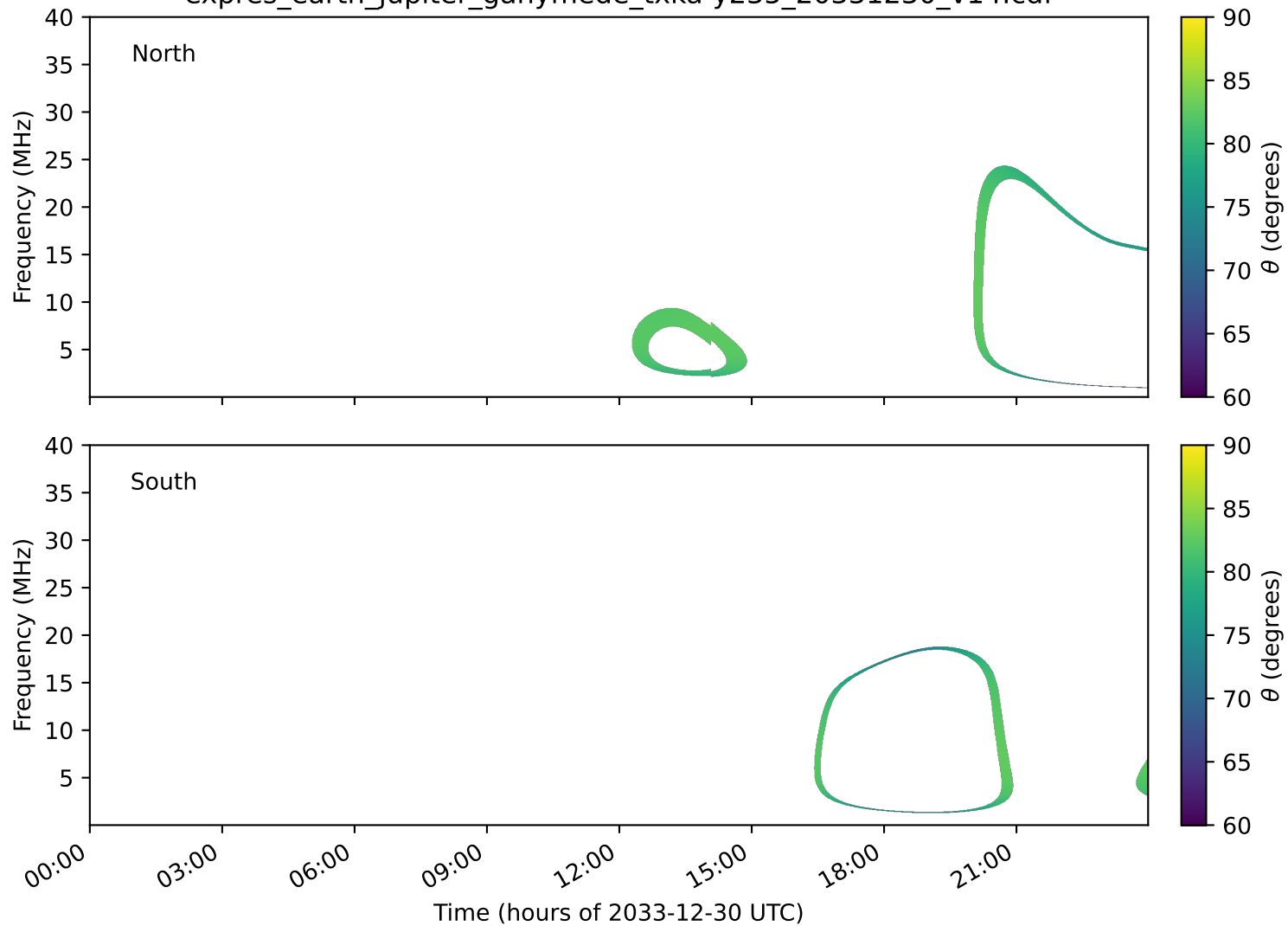
expres_earth_jupiter_ganymede_txka-y235_20331230_v14.cdf
