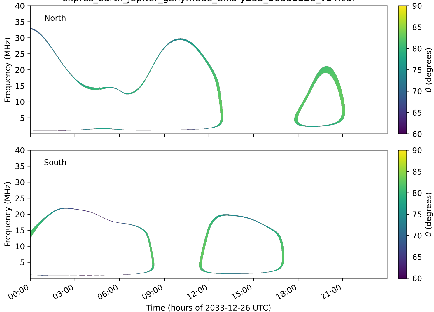
expres_earth_jupiter_ganymede_txka-y235_20331226_v14.cdf
