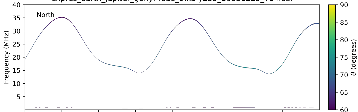
expres_earth_jupiter_ganymede_txka-y235_20331225_v14.cdf
